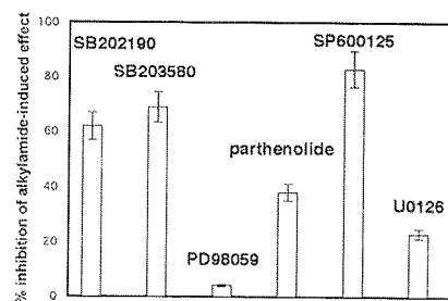
Fig. 8. Co-incubation with different kinase inhibitors incubated 1 h prior to monocyte/Mφs stimulation with 1/2 (5 μM). Concentrations used were twice IC 50 reported by manufacturer (Toocris Cookson Ltd.). Parthenolide were used at 5 μM. Shown is (%) inhibition (mean ± S.E.) of the 1/2-induced effect described in Fig. 3. Data are mean values (±S.E.) of four experiments (two different blood donors).
