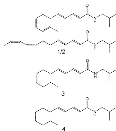
Fig. 3. Structures of the isolated alkylamides studied: (1/2) isomer pair dodeca-2 E ,4 E ,8 Z ,10 E -tetraenoic acid isobutylamide and dodeca-2 E ,4 E ,8 Z ,10 Z -tetraenoic acid isobutylamide, (3) dodeca-2 E ,4 E ,8 Z -trienoic acid isobutylamide, and (4) dodeca-2 E ,4 E -dienoic acid isobutylamide.
